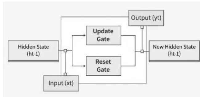
Figure 3. Prediction method with the GRU model.
