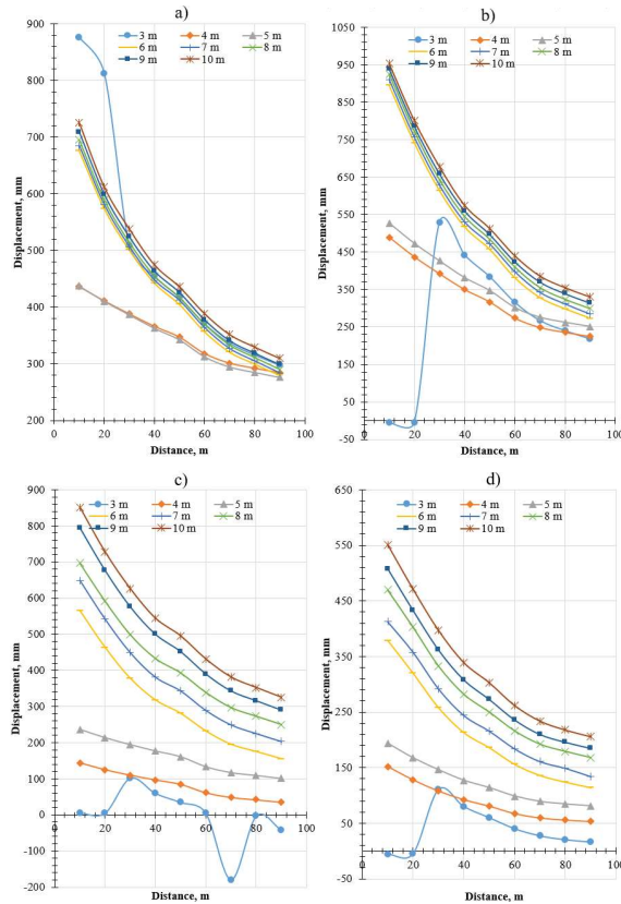
Fig. 11. Convergence of the roadway different narrow pillar width: a – roof sagging; b – displacement of solid coal side; c – floor heave; d – displacement of narrow coal pillar side.
