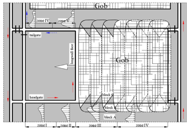
Fig. 3. Law of main roof collapse and characteristics of stress-deformation changes of the surrounding rock
