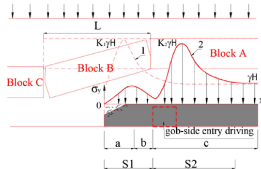
Fig. 4. Mechanical model of the "hanging-collapse" structure of the main roof and the stress distribution on the edge of coal seam
