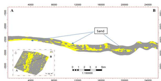
Fig. 16. Reconstruction of lake slope sand facies and lake floor sand facies
