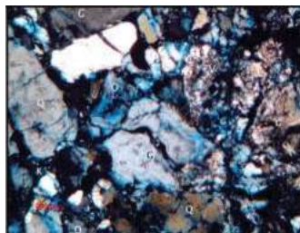
Sidewall core sample (at 3042m TVDs): arkose lithic sandstone with coarse grain, poor selectivity at well A1 (Q- quartz, P - Plagioclase)
