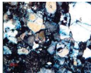
Sidewall core sample (at 3182.5m TVDs): arkose lithic sandstone with fine grain, medium selectivity at well B1 (Q- Quartz, P - Plagioclase, k-feldspar)
