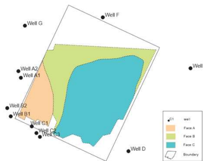
Fig. 10. Seismic facies map of sequence C
