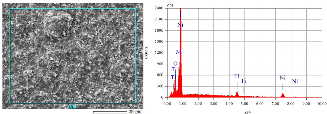
Figure 3-2 – EDX spectrum of Ni-TiO 2 composite plating samples created by normal square pulse current
