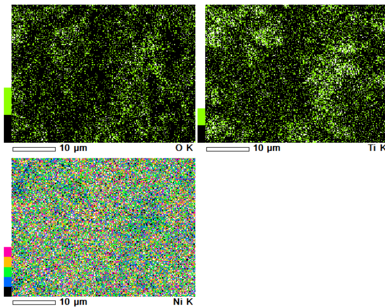
Figure 3-3 – SEM image – surface mapping of the Ni- \text{TiO}_2 coating
