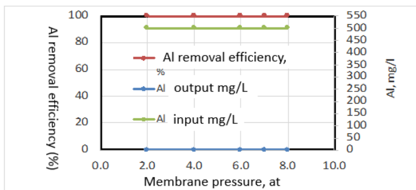
Picture 3-3 – Al removal efficiency
