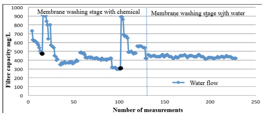
Picture 3-1 – The efficiency of membrane washing process
