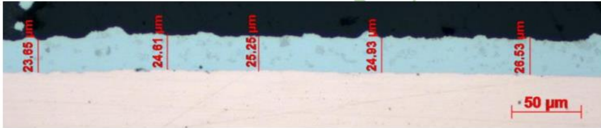
Figure 3-3 – Photograph of coating thickness Ni- \text{TiO}_2
