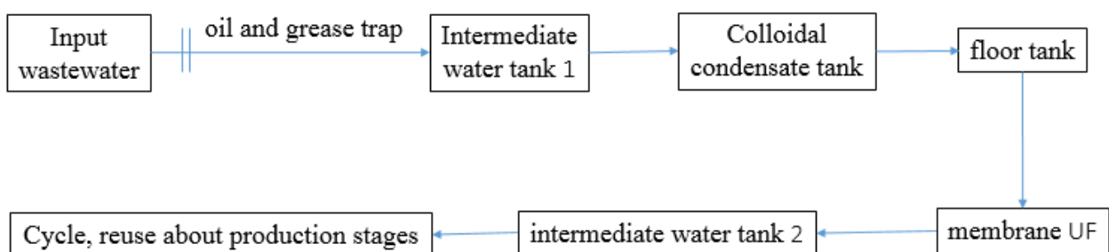
Picture 2-1 – Diagram of wastewater treatment system
