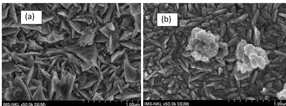
Figure 3-5 – SEM image of Ni (a) and Ni-nano TiO 2 (b) coatings
