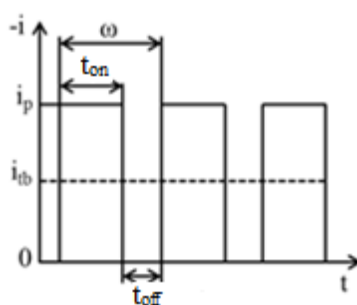
Figure 1-1 – Normal square pulse diagram
