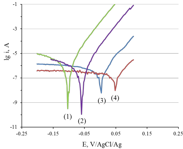
Figure 3-6 – Tafel lines of nickel-plated samples in 3.5% NaCl solution
