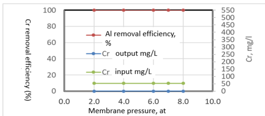
Picture 3-4 – Cr removal efficiency
