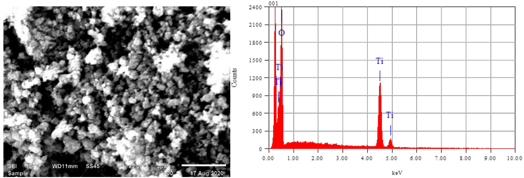
Figure 3-1 – SEM images and EDX spectra of TiO 2 particles
