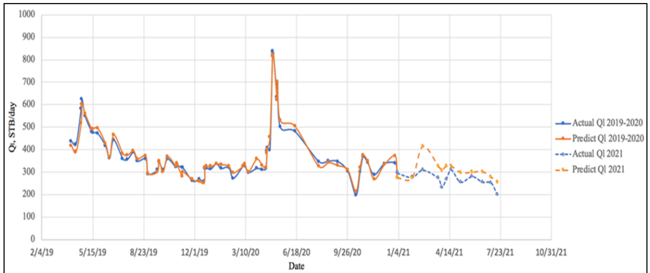
Figure 7. Comparing predicted production flow rate by the ANN model and actual data of well 01 in 2 production period (2019-2020 and 2021).
