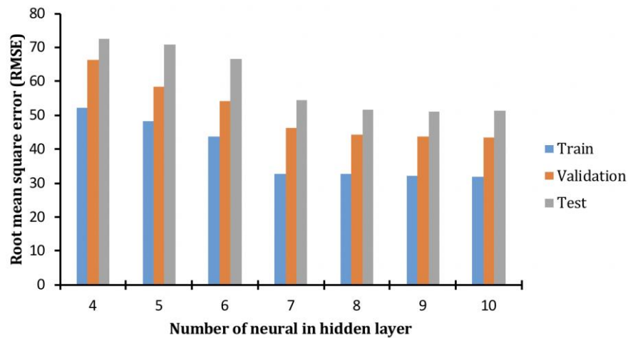
Figure 4. Results of root mean square error (RMSE) with different number of neural in the hidden layer.
