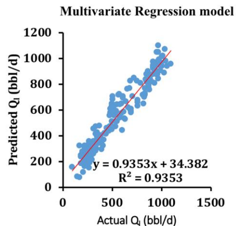
Figure 6. Cross plot of oil flow rate for Multivariate Regression model (Predicted Q_i ).
