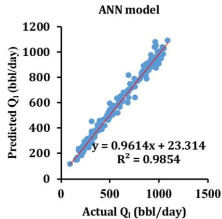
Figure 5. Cross plot of oil flow rate for ANN model (Predicted Q_i ).
