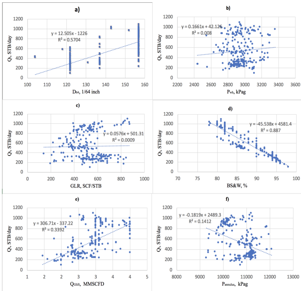
Figure 1. Correlations between production flow rate ( Q_1 ) and a) choke size; b) wellhead pressure ( P_{wh} ); c) ratio of gas to liquid (GLR); d) Free water, sediment and emulsion (BS&W); e) injected gas lift rate Q_{glift} ; f) injected gas lift pressure ( P_{annulus} ).
