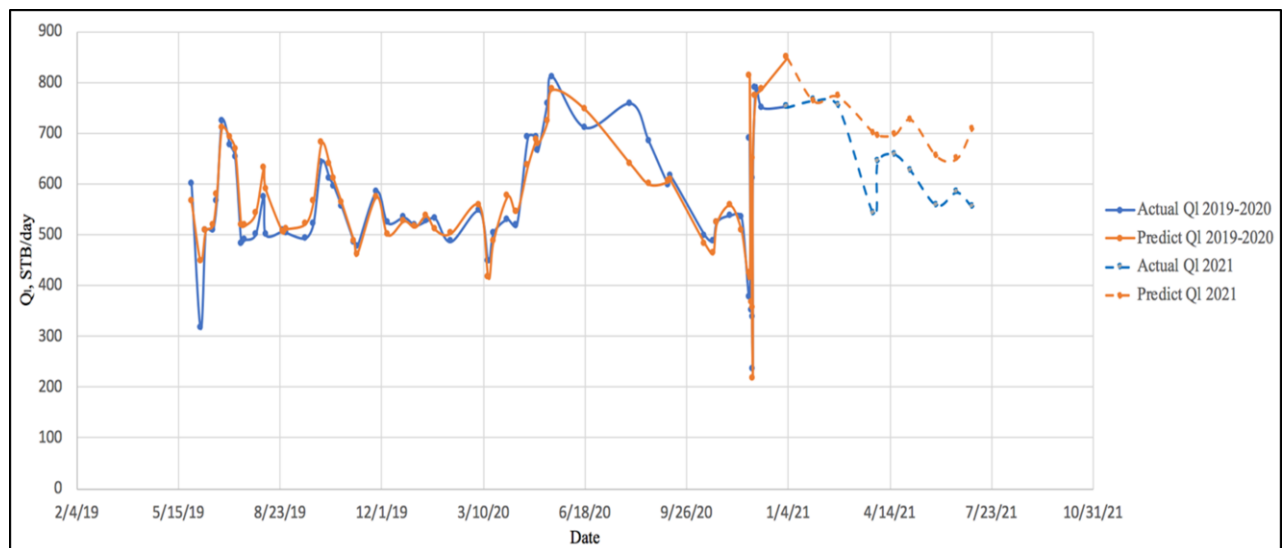
Figure 8. Comparing predicted production flow rate by the ANN model and actual data of well 05 in 2 production period (2019-2020 and 2021).
