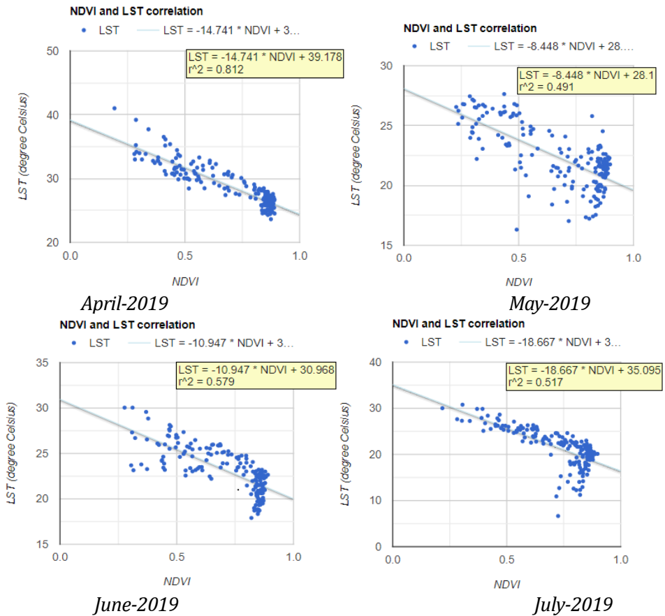
Figure 6. LST-NDVI correlation.
