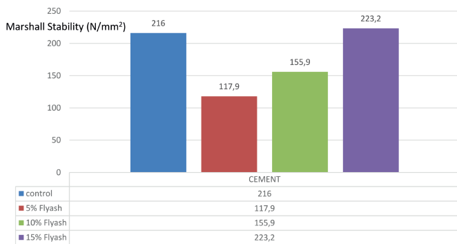
Fig. 1 Marshall stability test result of asphalt mixed with different percentages of fly ash
