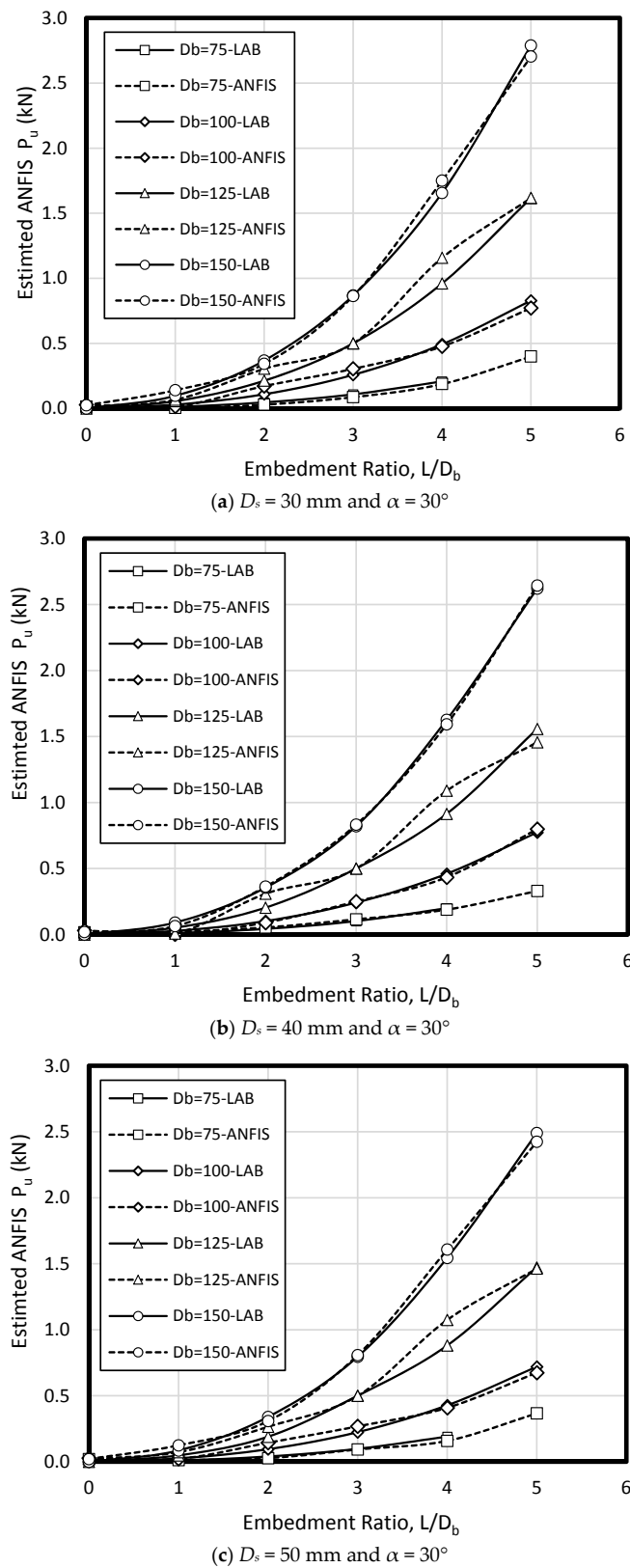
Figure 12. P_u for various D_s , D_b , and L/D_b in laboratory model and predicted from ANFIS when \alpha = 30^\circ in loose sand.
