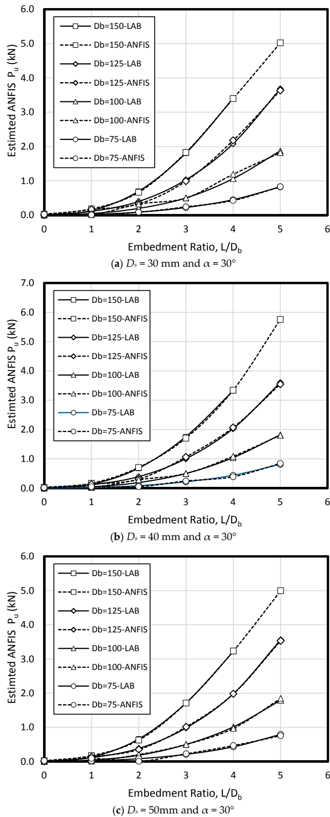
Figure 9. P_u for various D_s , D_b , and L/D_b in laboratory model and predicted from ANFIS when \alpha = 30^\circ in dense sand.
