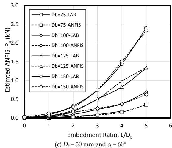
Figure 14. P_u for various D_s , D_b , and L/D_b in laboratory model and predicted from ANFIS when \alpha = 60^\circ in loose sand.
