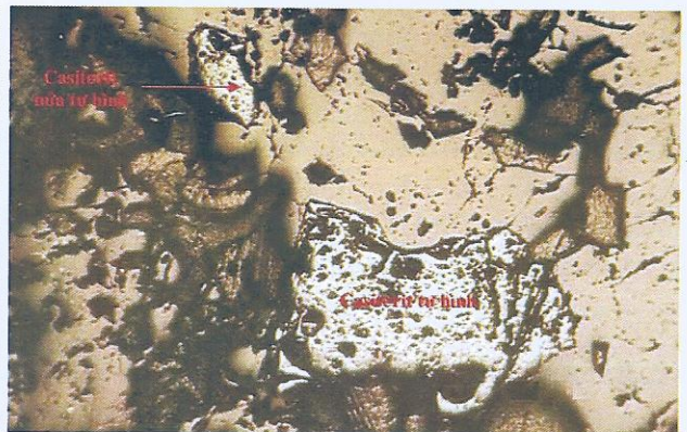
Figure 7. The mineragraphic sample KTH.5DSx40, cassiterite.
