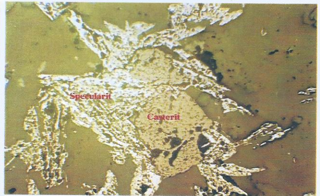
Figure 5. The mineragraphic sample KT.2529 /3x100, Specularite replaces and reattaches cassiterite.
