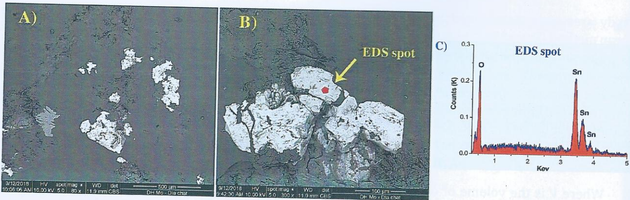
Figure 8. SEM-EDS analysis shows that the presence of minerals of Sn in the sample. A-B) SEM images of tin mineral; C) EDS spot of tin mineral.
