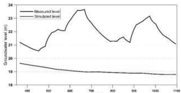
Fig7. Comparison between measured level and simulated level of groundwater
