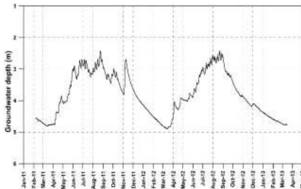
Fig2. Groundwater level variations in irrigated land
